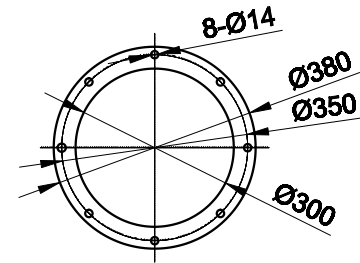
Inlet Flange (A View)
