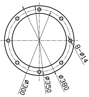
Inlet Flange (A View)
