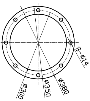
Inlet Flange (A View)
